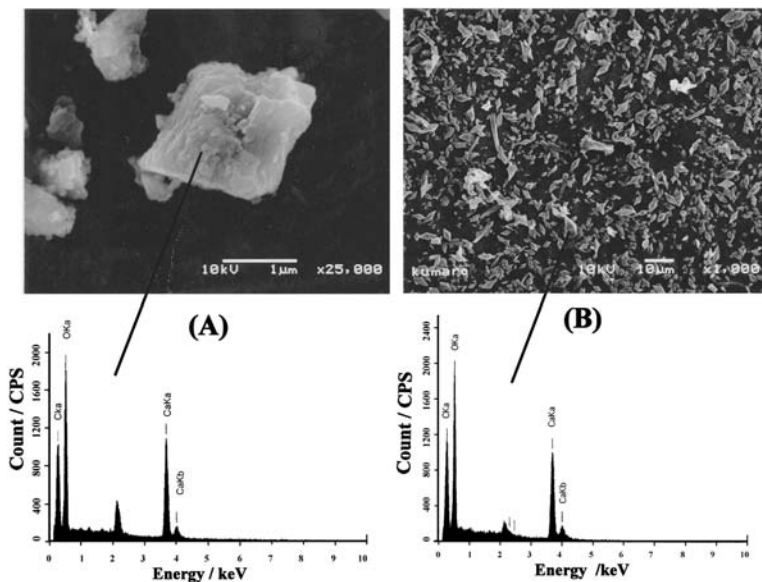
Fig. 11 Examples of SEM photographs with point analyses by EDX of the substance on Nuclepore membrane filter (0.1 \mu m pore size) after having filtered the Kumanoyu hot spring water. (A) : Source (2005) ( \times 25,000) and (B) : Open-air bath (2005) ( \times 1,000).
