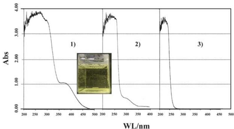
Fig. 8 Change of absorption spectrum of the water 1) made by conduction H_2S into the water after dissolving elemental sulfur in distilled water. 2) and 3) are the spectra of the water after having left it more for 5 and 15 days, respectively.
