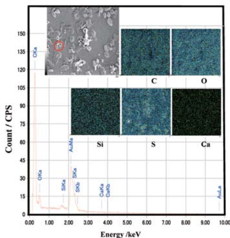
Fig. 13 Example of SEM mapping image with point analyses by EDX of the substance on Nuclepore membrane filter (0.1 \mu m pore size) after having filtered the Kumanoyu hot spring water.
