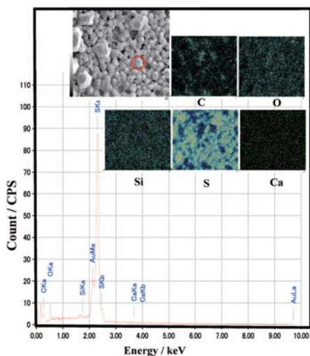
Fig. 12 Example of SEM mapping image with point analyses by EDX of the substance on Nuclepore membrane filter (0.1 \mu m pore size) after having filtered the Kunimi hot spring water.
