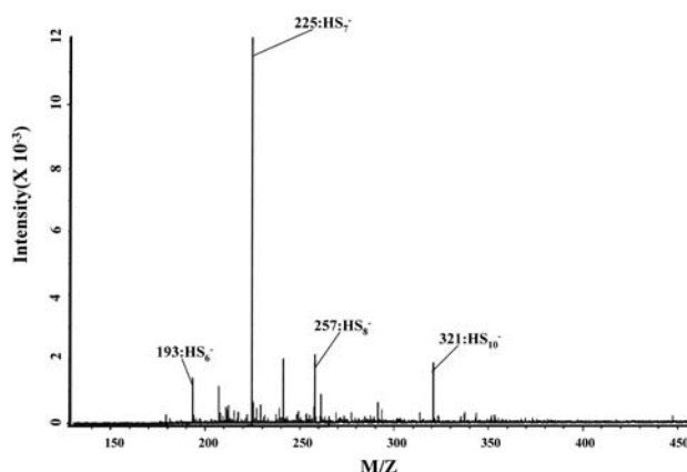
Fig. 9 ESI-MS spectra of water colored in green after having left the water of source of Kumanoyu hot spring for a few days.
