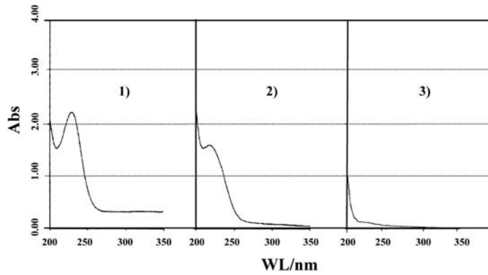
Fig. 6 Change of absorption spectrum of the water 1) colored in green after having left the water of source of Kunimi hot spring for a few days. 2) and 3) are the spectra of the water after having left it more for 5 and 15 days, respectively.
