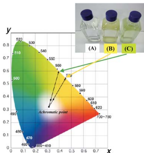
Fig. 14 Calorimetric data shown on the xy-chromaticity diagram established by Commission Internationale d'Éclairage (CIE) in 1931. Photographs are (A) : distilled water, (B) : the water containing polysulfide ion and (C) : the water added CaCO 3 (average particle size ≒ 80 nm) into (B).
