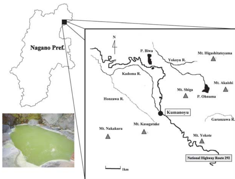
Fig. 2 A location map of Kumanoyu hot spring in Nagano Prefecture and a photograph of the open-air bath of Kumanoyu hot spring.
